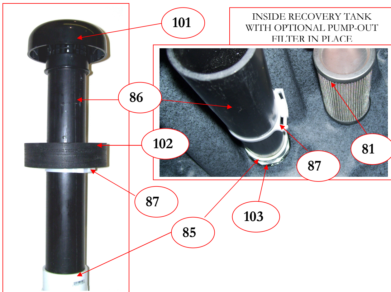
VACUUM SHUTOFF ASSEMBLY
