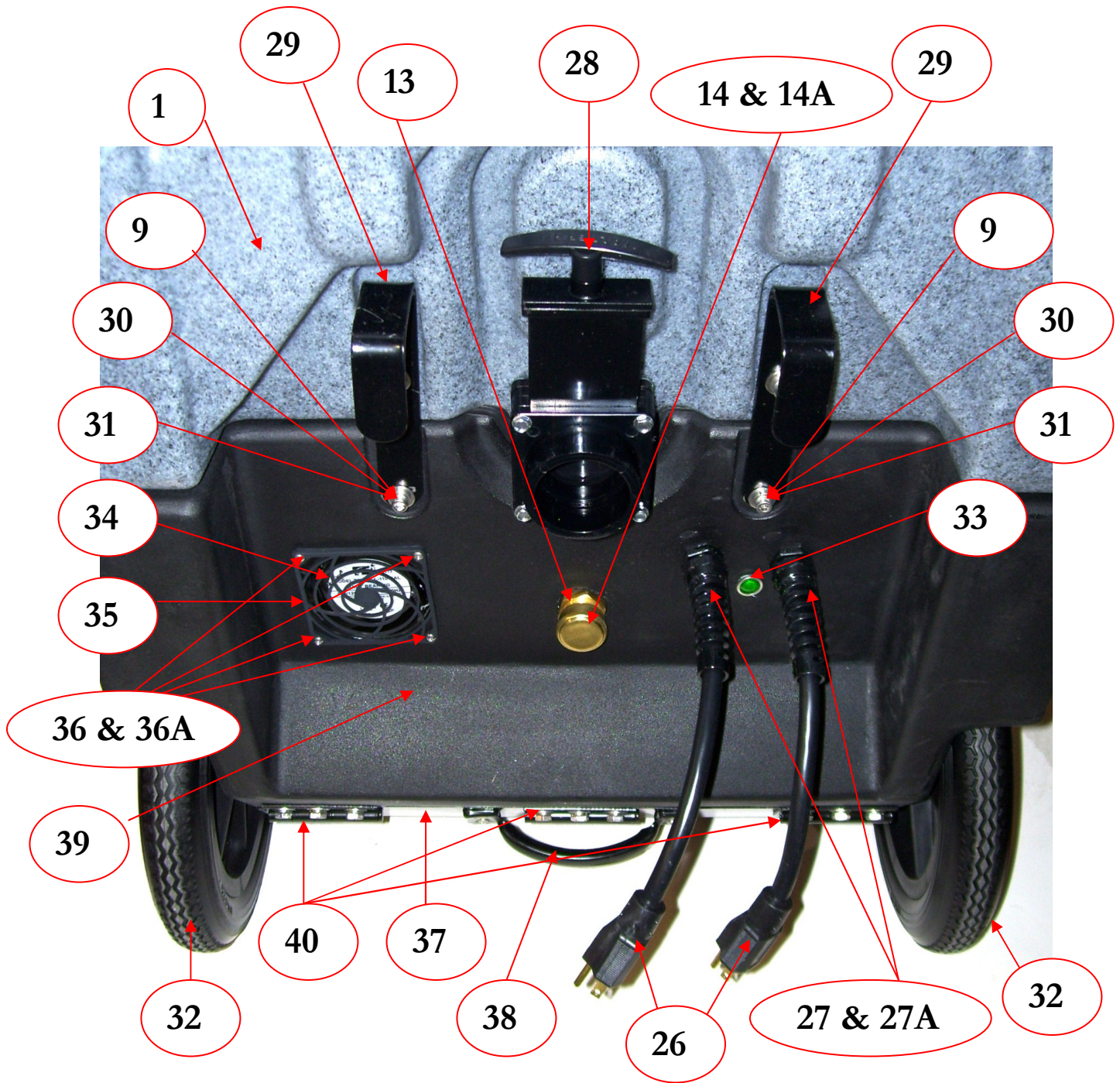
REAR VIEW – BASE, BASE SKIRT & RECOVERY TANK Shown with optional Pump-Out
